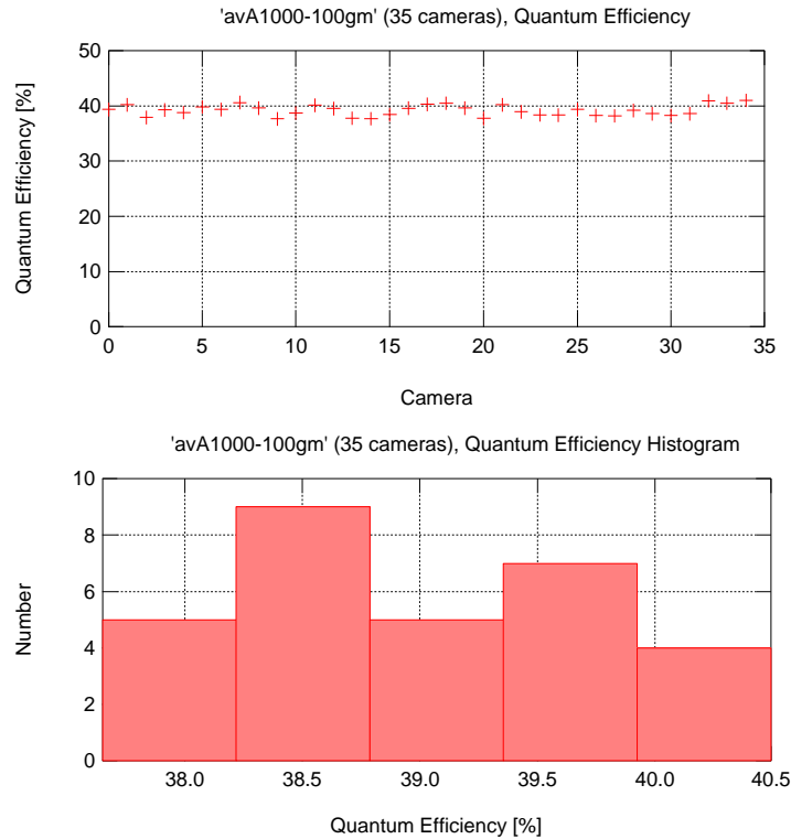
Figure 2: Total Quantum Efficiency (QE)
