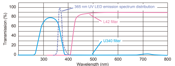
Filter characteristic vs. UV LED emission spectrum distribution
