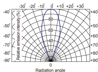
Directional pattern of UV light LED
